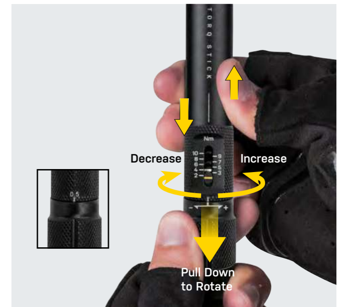
Rotate a half turn for 0.5Nm adjustment
