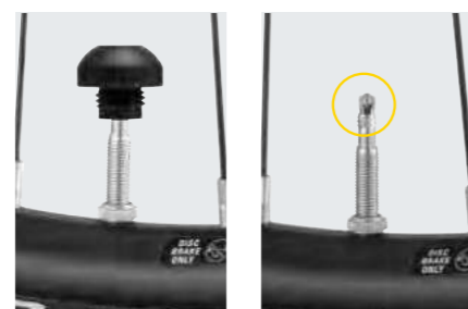
Built-in tool (PCT Cap) to tighten or remove two-piece Presta valve cores
