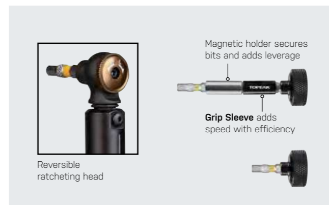
The pro version provides multiple combination choices to repair or maintain your bike.
