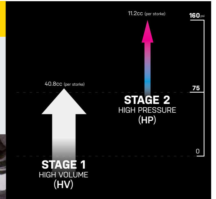
Stage 2 : High Pressure (75 - 160 psi)
